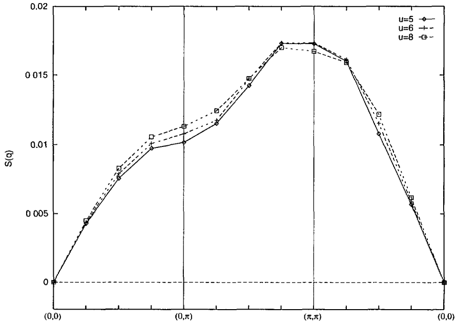
Fig. 2. — Spin-spin correlation S(q) for an 8 \times 8 -system for U ranging from 5 to 8, 50 particles (doping 0.21) t_p = -0.22 .
